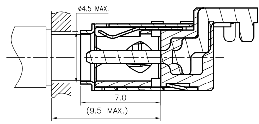
REFERENCE MATING DRAWING
